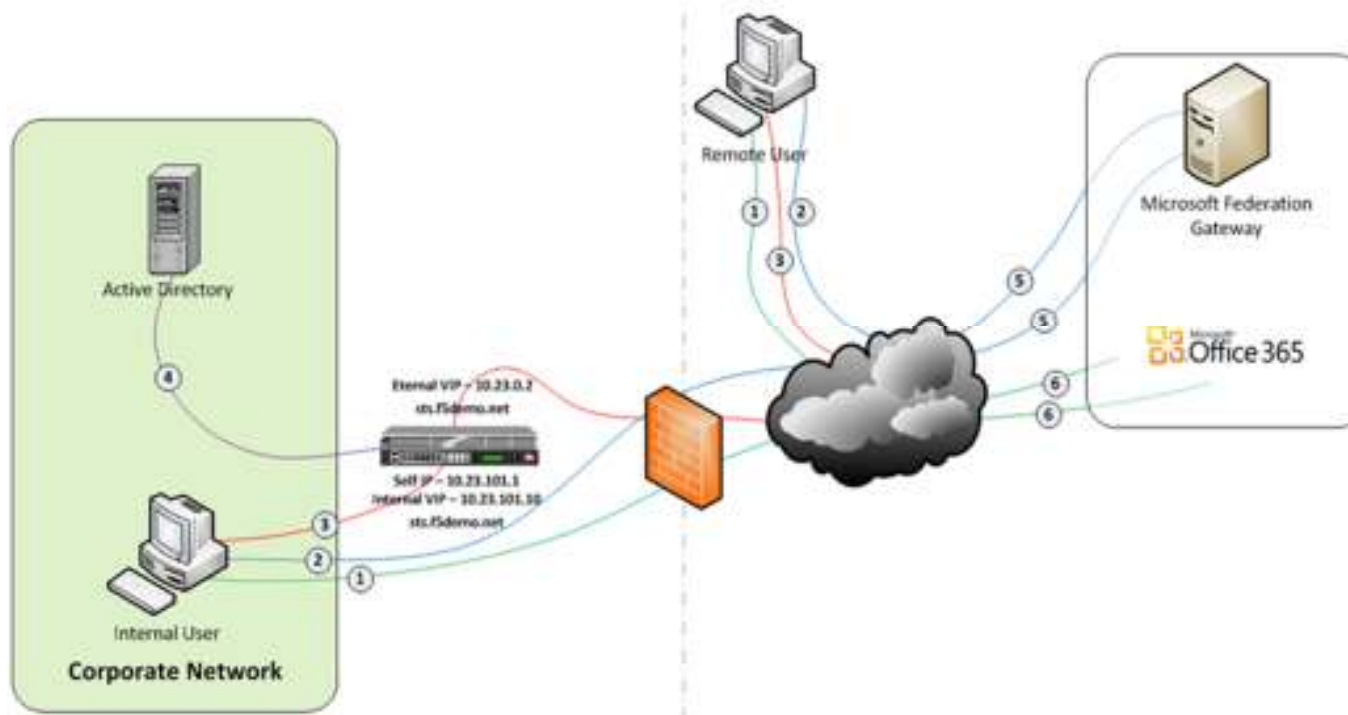
Figure 3 – BIG-IP with APM replacing the entire ADFS infrastructure
